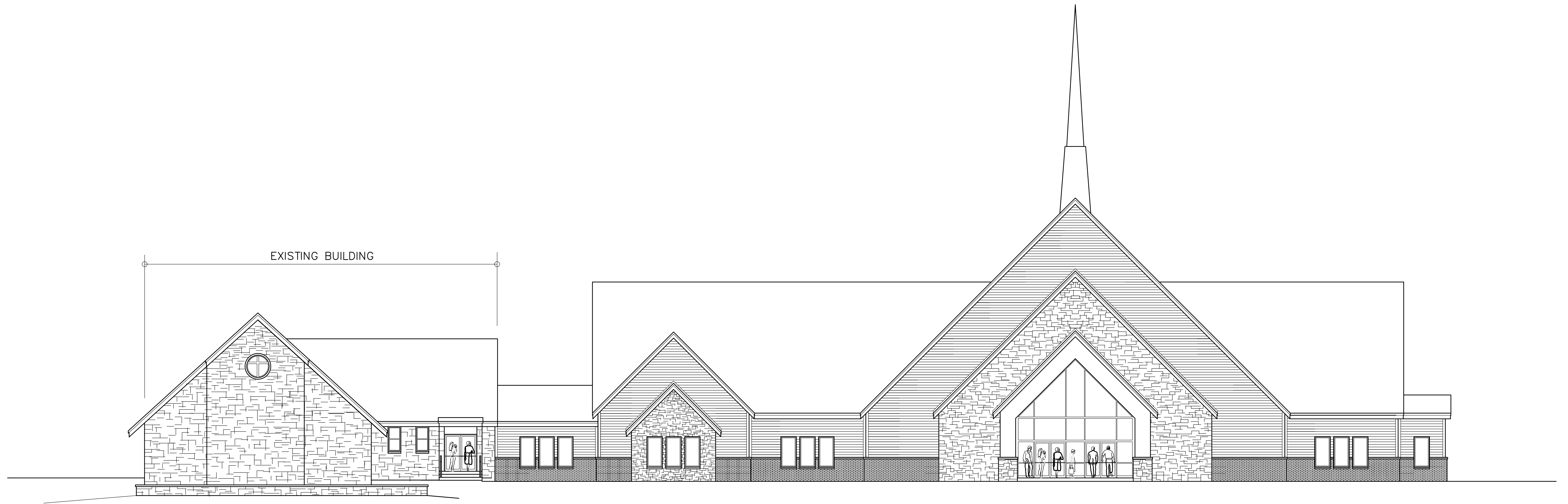
NORTH ELEVATION
